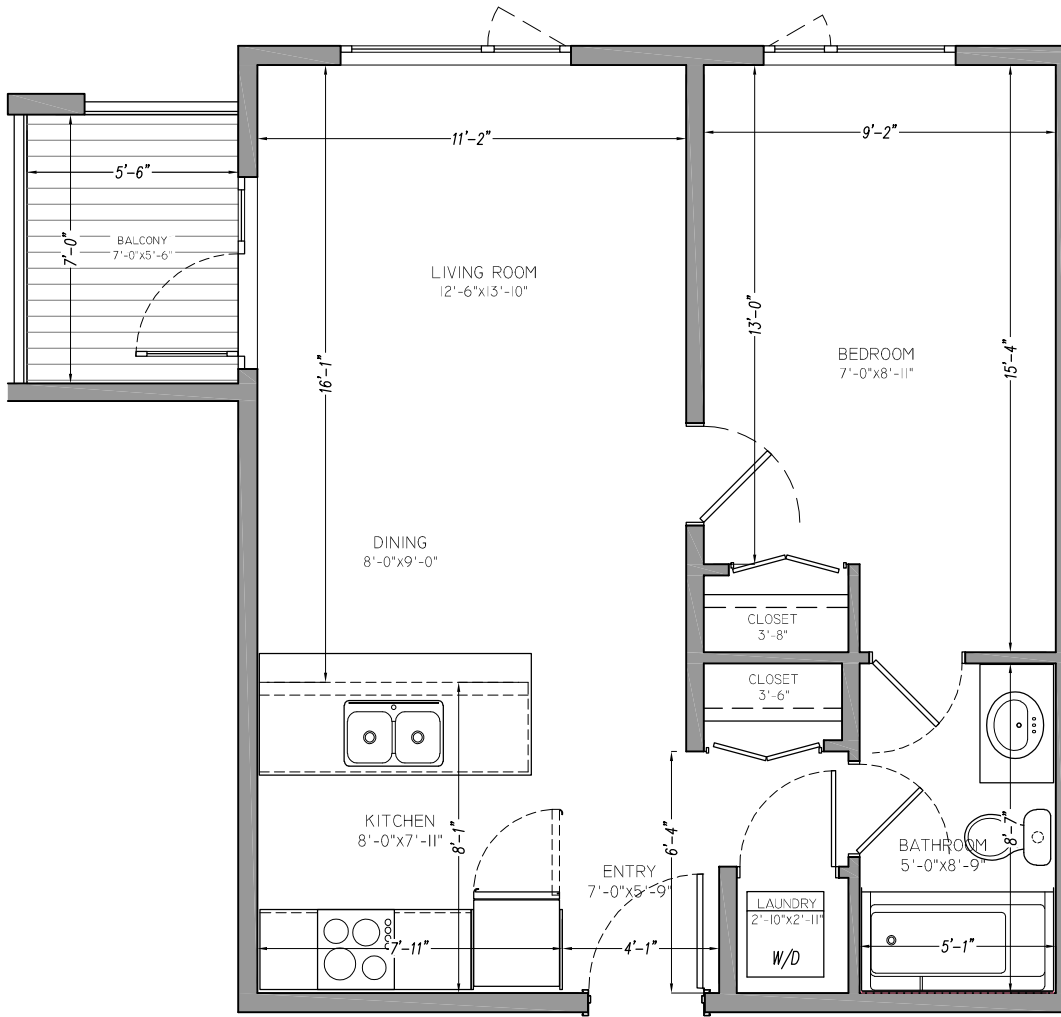
TYPICAL UNIT "D"
